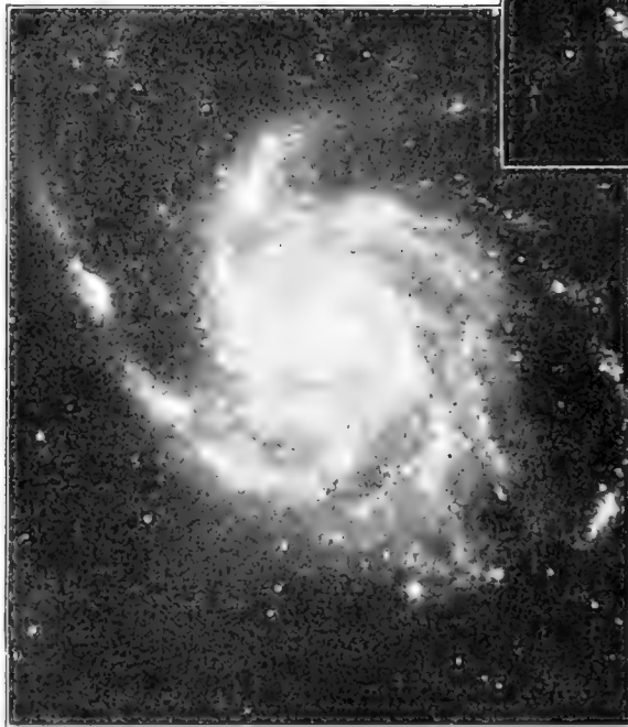
Another photograph of the same nebula, taken with the sixty-inch reflector of the Mt. Wilson Solar Observatory. Time of exposure, seven hours, thirty minutes. Comparison shows the greater detail in the lower photograph
